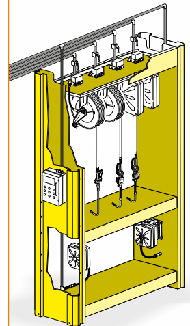
1 Universal drillings for application of accessories
